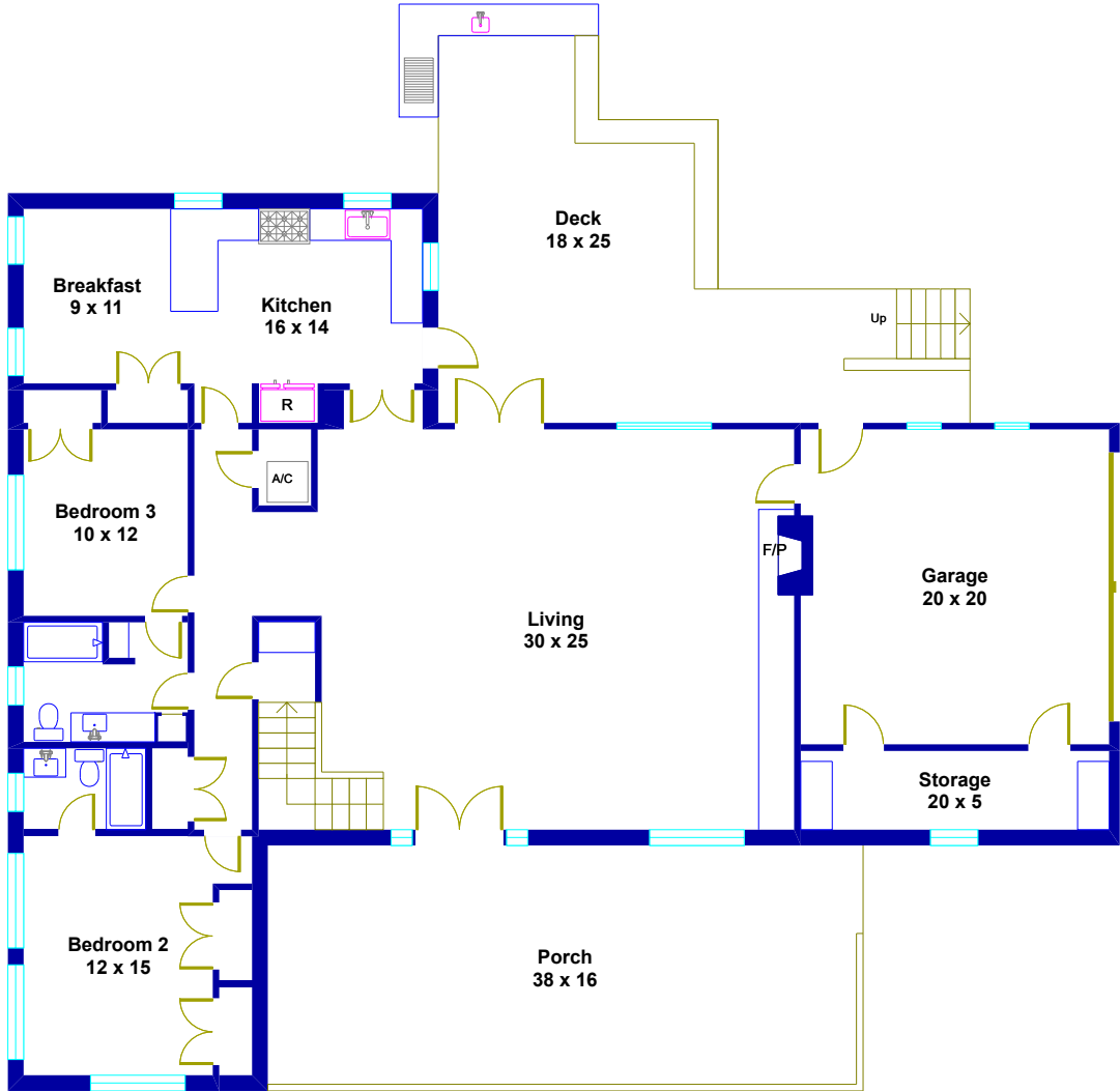
House First Floor
